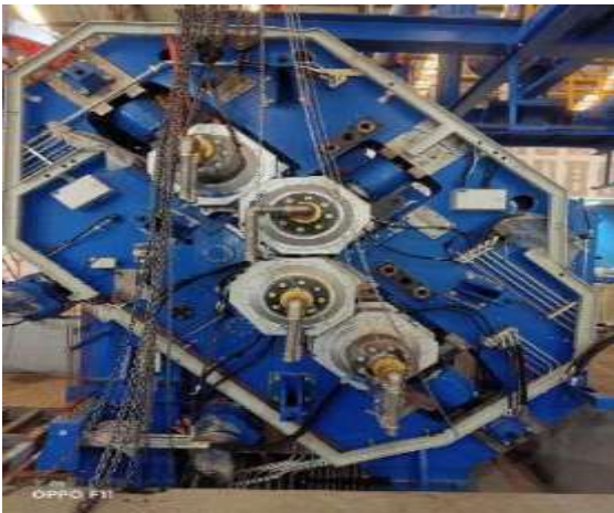
Lifting and setting of steel calendar machine at Gajah Tunggal Project
